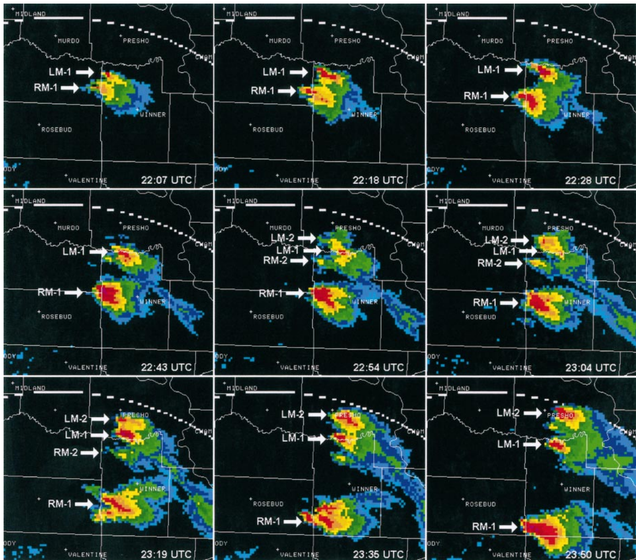
FIG. 8. WSR-88D base reflectivity from the KLNx radar on 24 Jul 2000. Times shown are 2207, 2218, 2228, 2243, 2254, 2304, 2319, 2335, and 2350 UTC. Arrows are as follows: RM1 and LM1 are the primary right- and left-moving storms, respectively, and RM2 and LM2 appear to be new storms associated with LM1.
